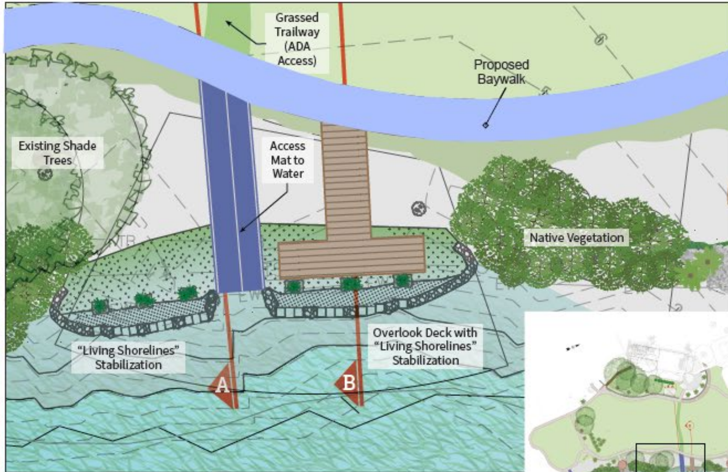
Proposed Plan for Bay Overlook and Living Shoreline
