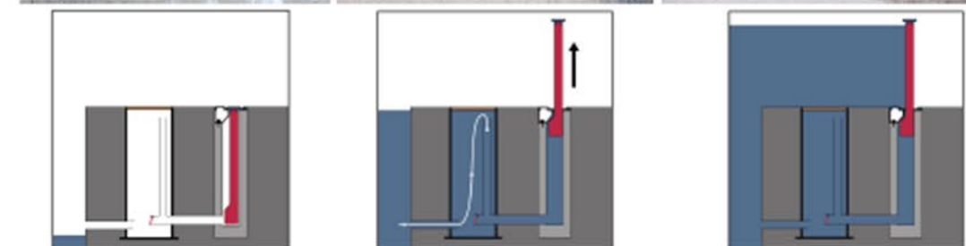
Self Closing Flood Barrier: Below-ground gate rises up automatically during high water to protect Community Center from storm waves
