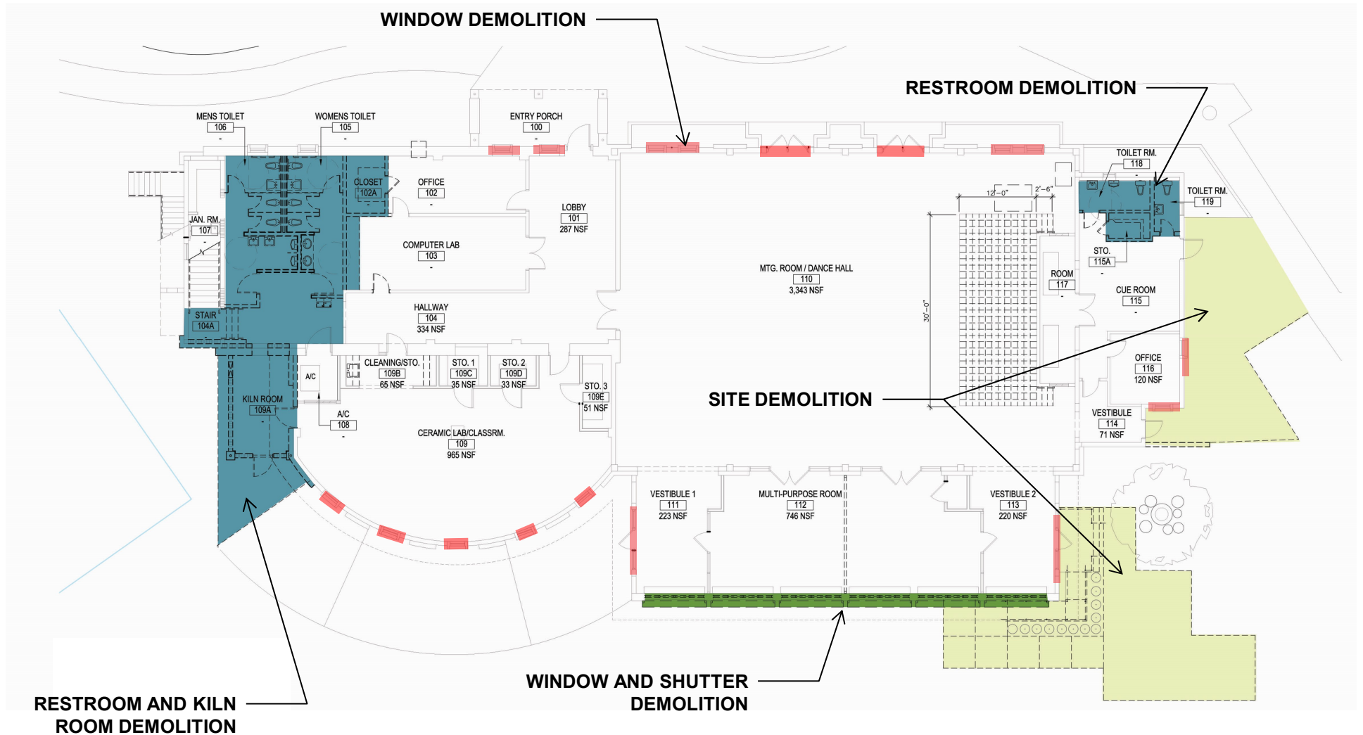
1 ST FLOOR DEMOLITION PLAN
